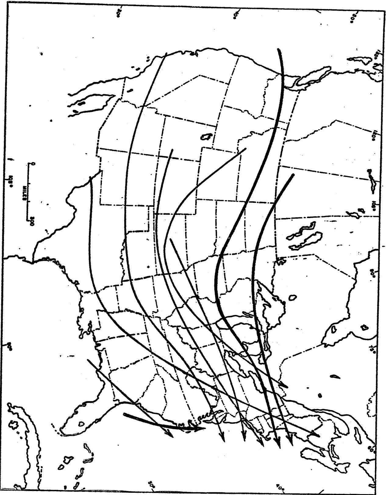
FIGURE 5.4. Most frequent tracks of low pressure systems. The heavier lines indicate more frequent occurrence.
